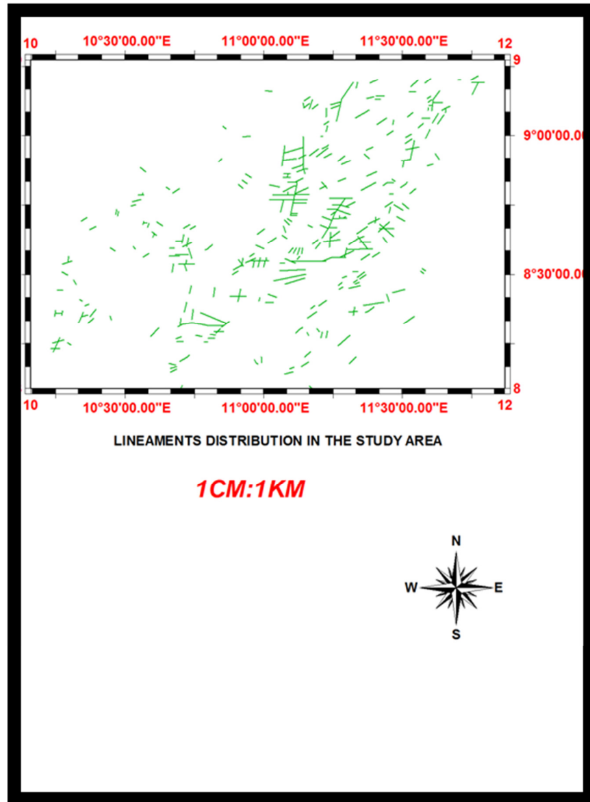
Figure 3. Lineament map of the study area.
