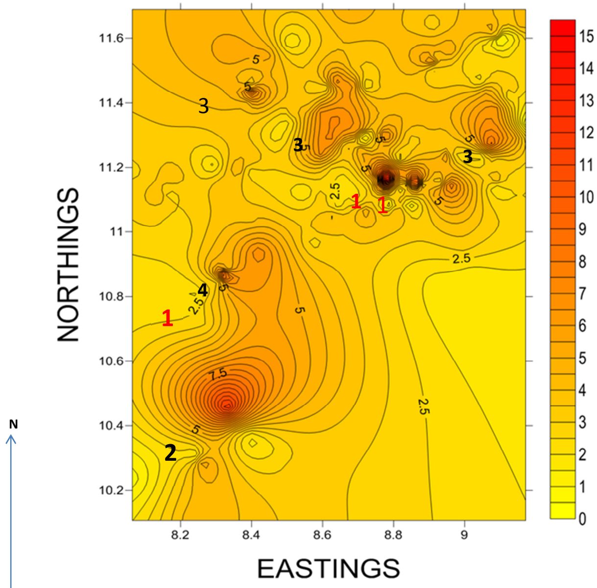
Figure 6. Lineament density map of the study area.
