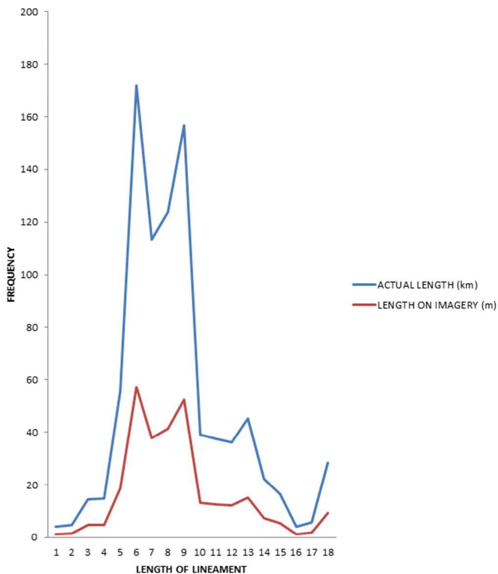
Figure 9. Relationship between the actual length of lineaments and lineaments on imagery.
