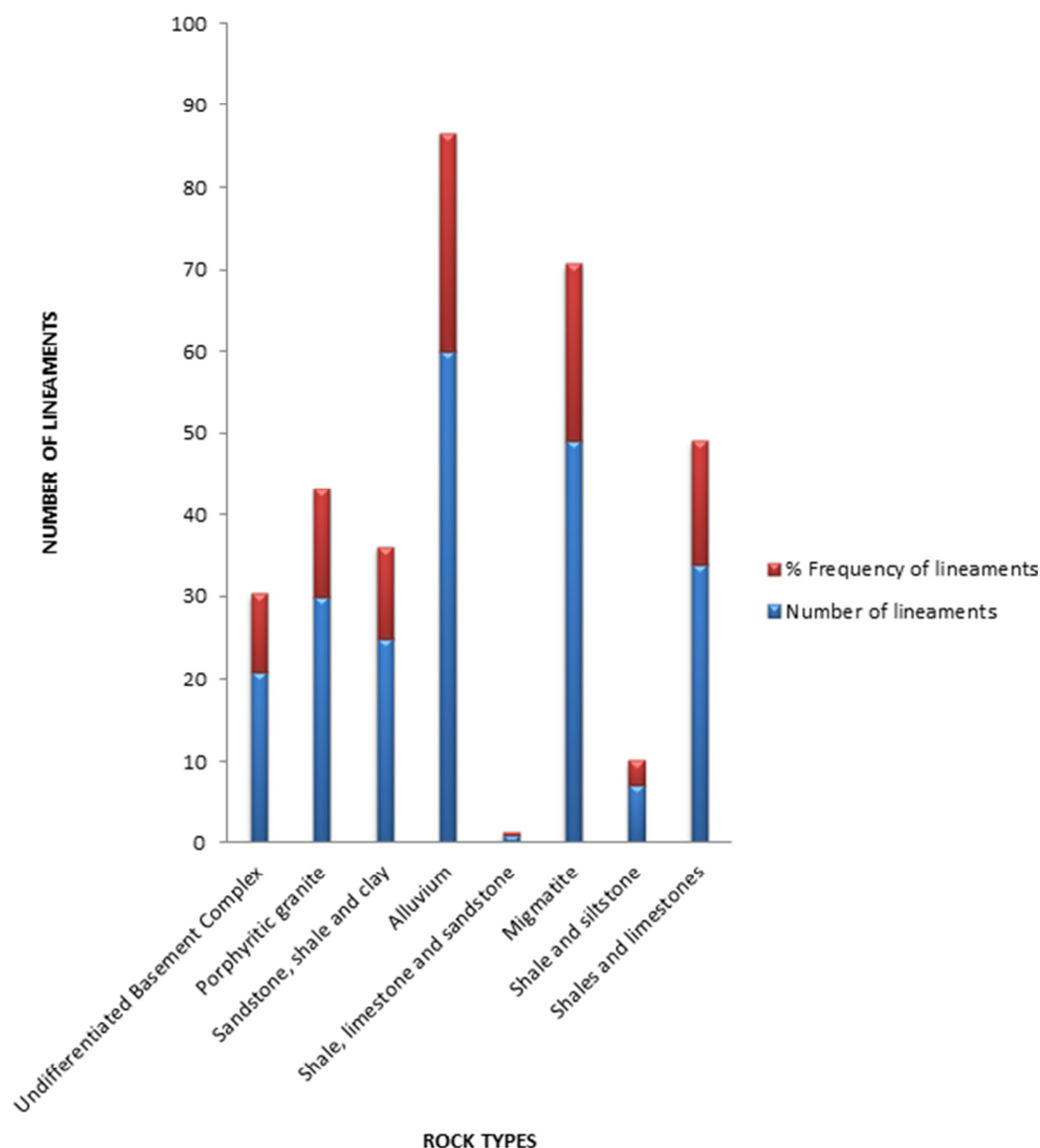
Figure 4. Distribution of lineaments over the rocks in the study area.
