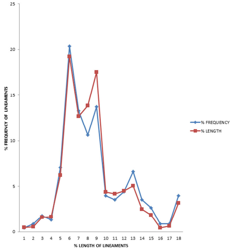
Figure 5. Relationship between percentage frequency of lineaments and percentage length of lineament.
