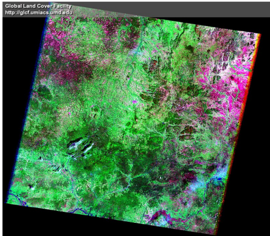
Figure 1. LANDSAT imagery of the study area.
