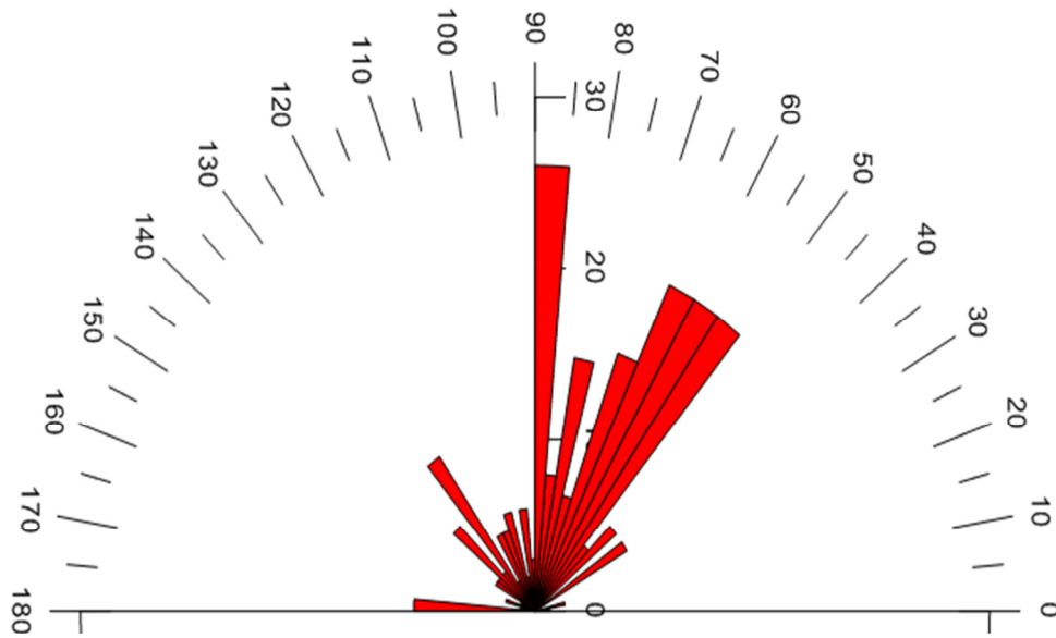
Figure 7. Rose Diagram from Lineaments mapped from Landsat imagery (N = 226).
