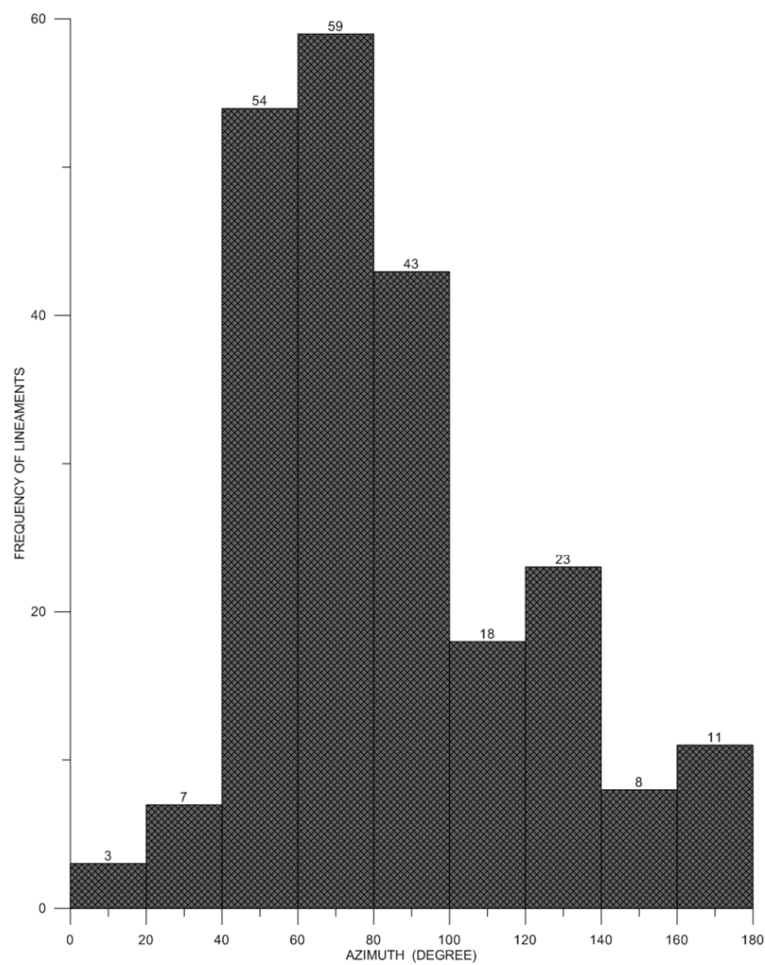
Figure 8. Histogram obtained from azimuth data of the area.
